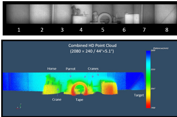
LCPG steering used to stitch 8 fields of view in flash lidar.
